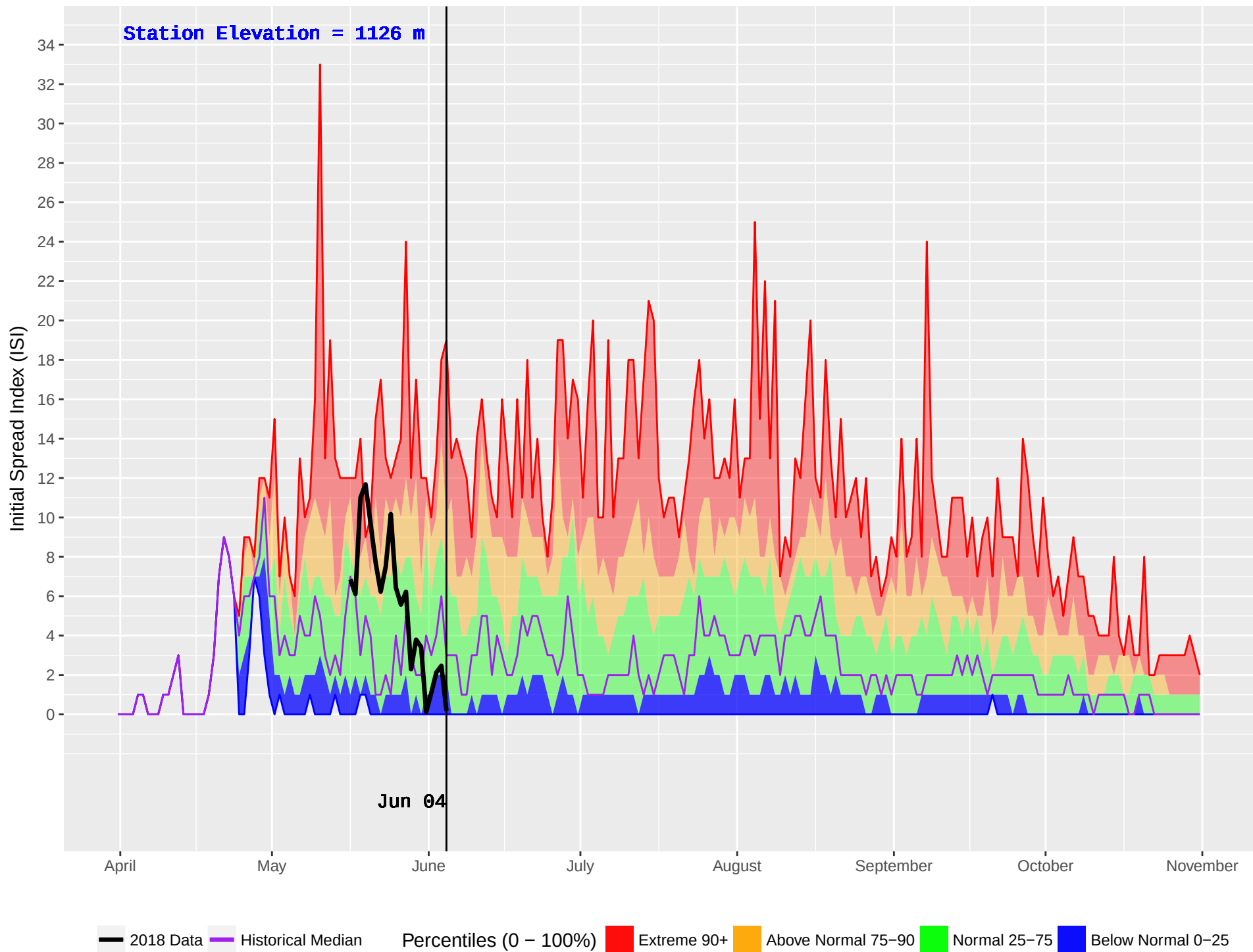
BLACKPINE (148) : Historical (1980–2016) and Current (2018) Noon Initial Spread Index (ISI)
