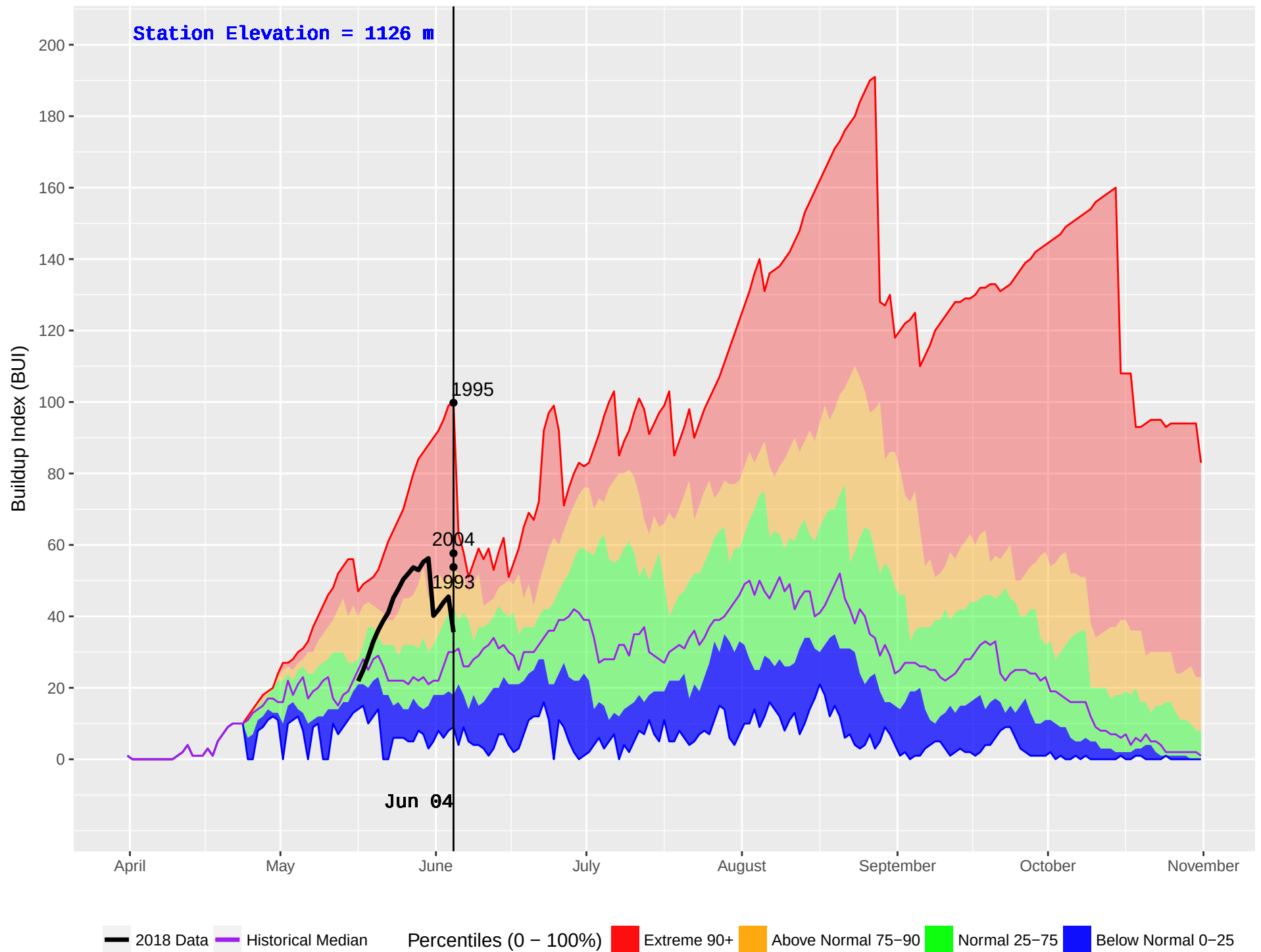
BLACKPINE (148) : Historical (1980–2016) and Current (2018) Noon Buildup Index (BUI)
