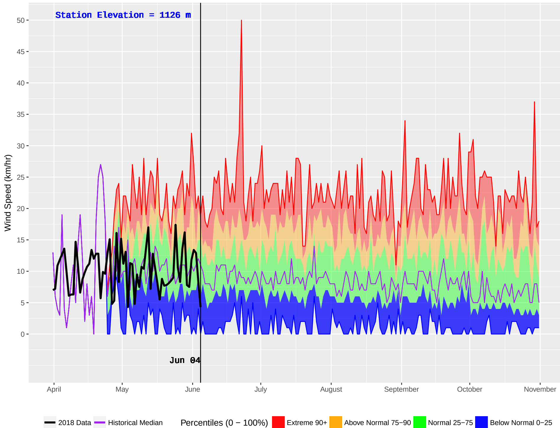
BLACKPINE (148) : Historical (1980–2016) and Current (2018) Noon Wind Speed
