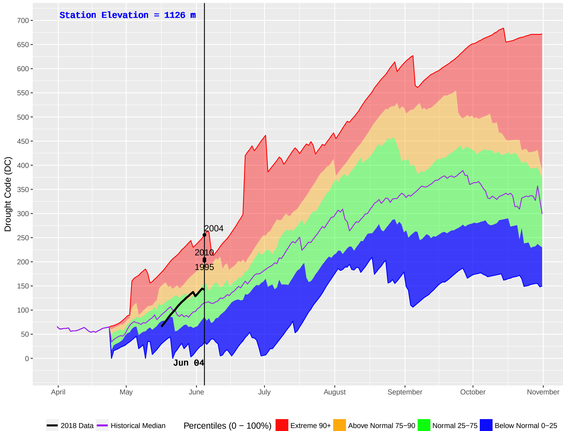
BLACKPINE (148) : Historical (1980–2016) and Current (2018) Noon Drought Code (DC)
