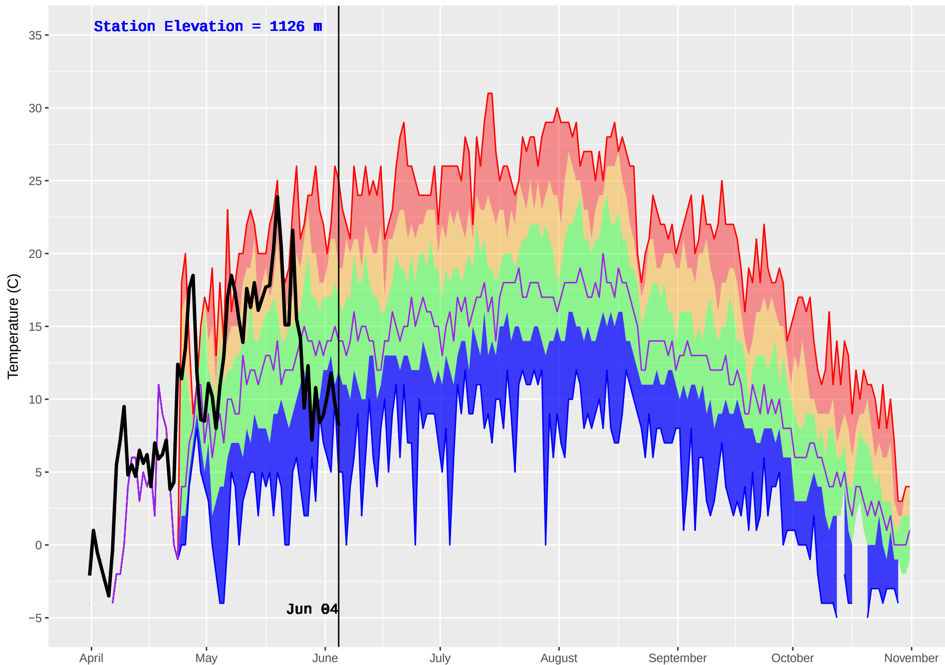
BLACKPINE (148) : Historical (1980–2016) and Current (2018) Noon Temperature
