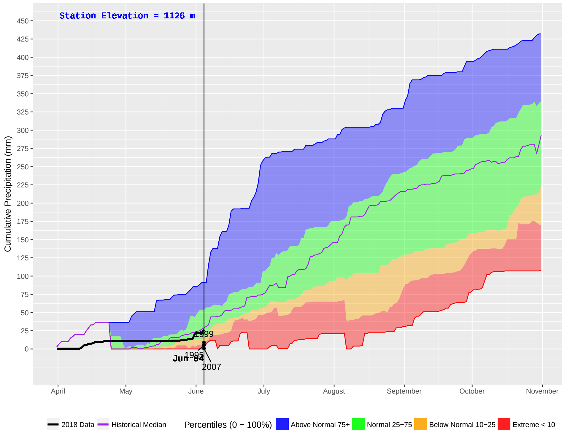
BLACKPINE (148) : Historical (1980–2016) and Current (2018) Noon Cumulative Precipitation
