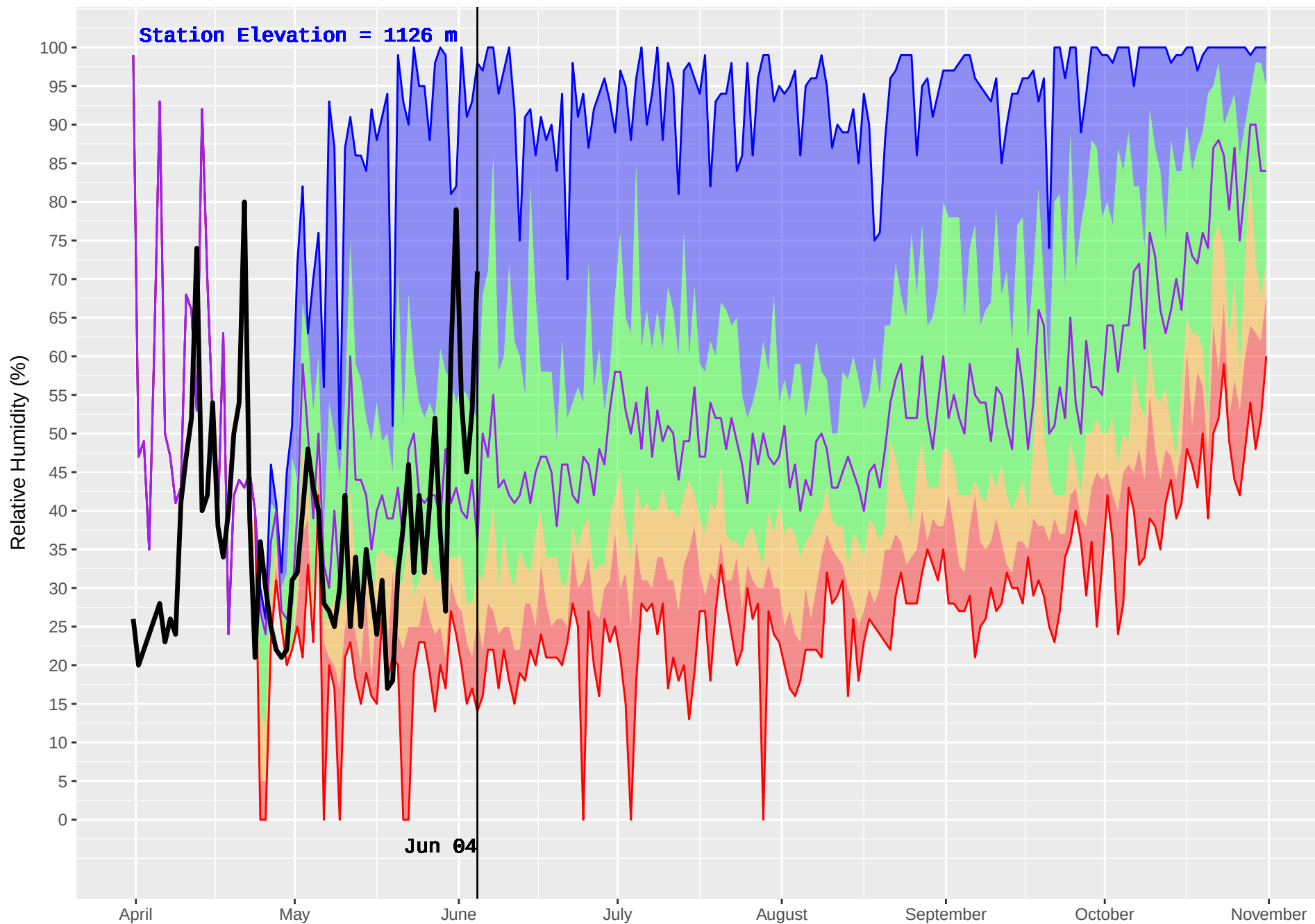
BLACKPINE (148) : Historical (1980–2016) and Current (2018) Noon Relative Humidity
