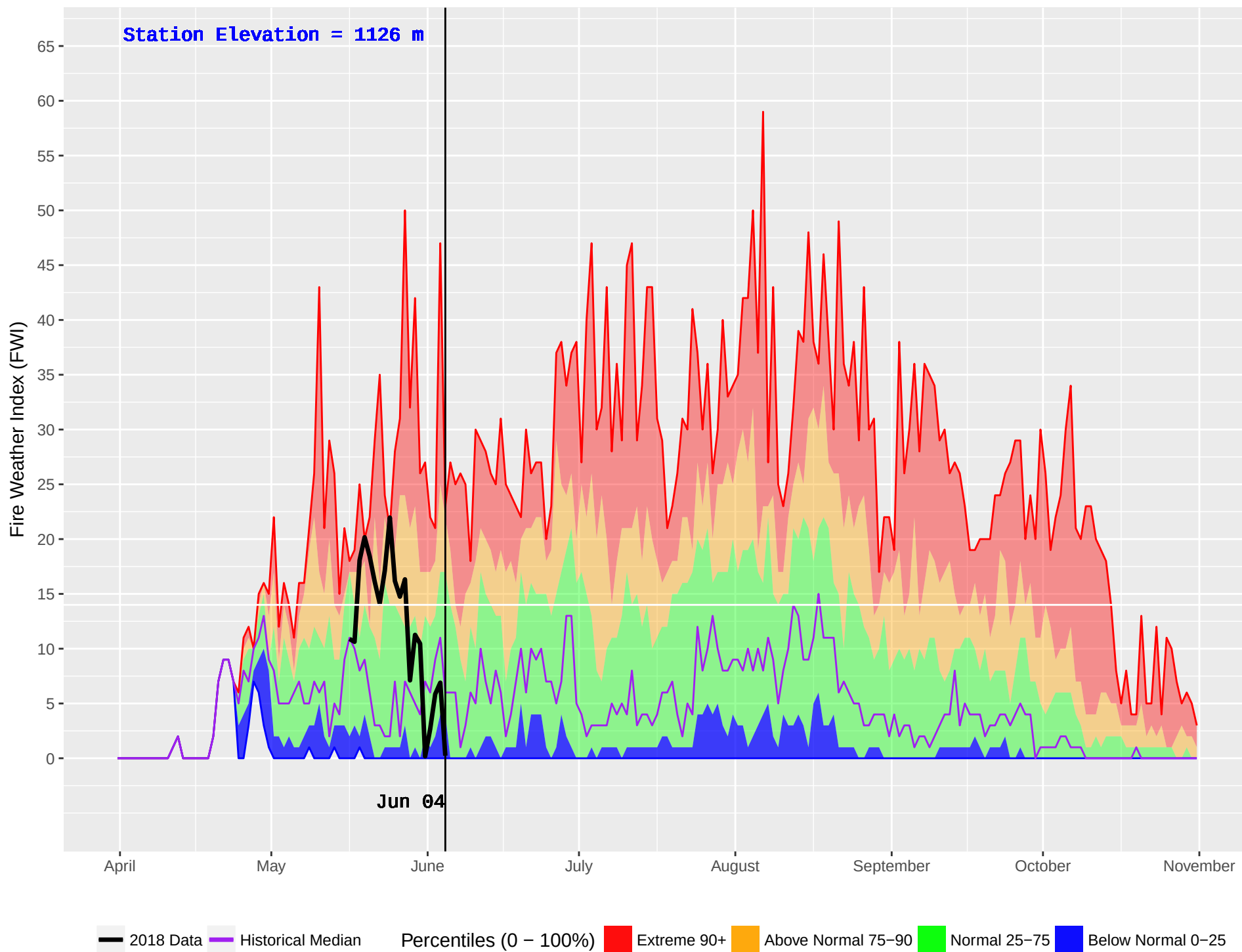
BLACKPINE (148) : Historical (1980–2016) and Current (2018) Noon Fire Weather Index (FWI)
